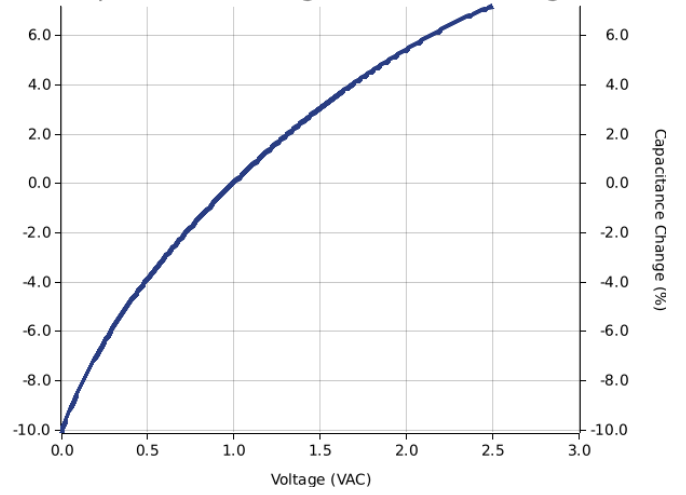
Capacitance Change versus AC Voltage
