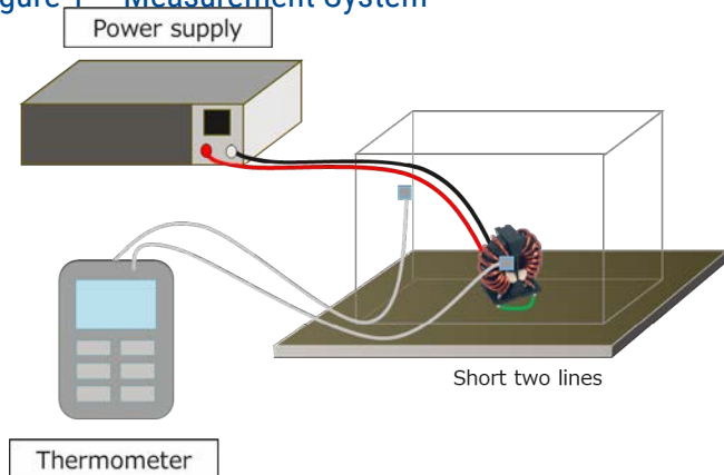
Figure 1 – Measurement System
