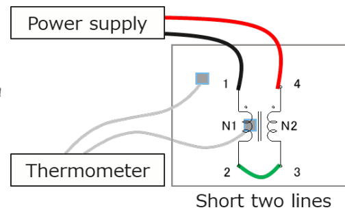
Figure 2 - Schematics
